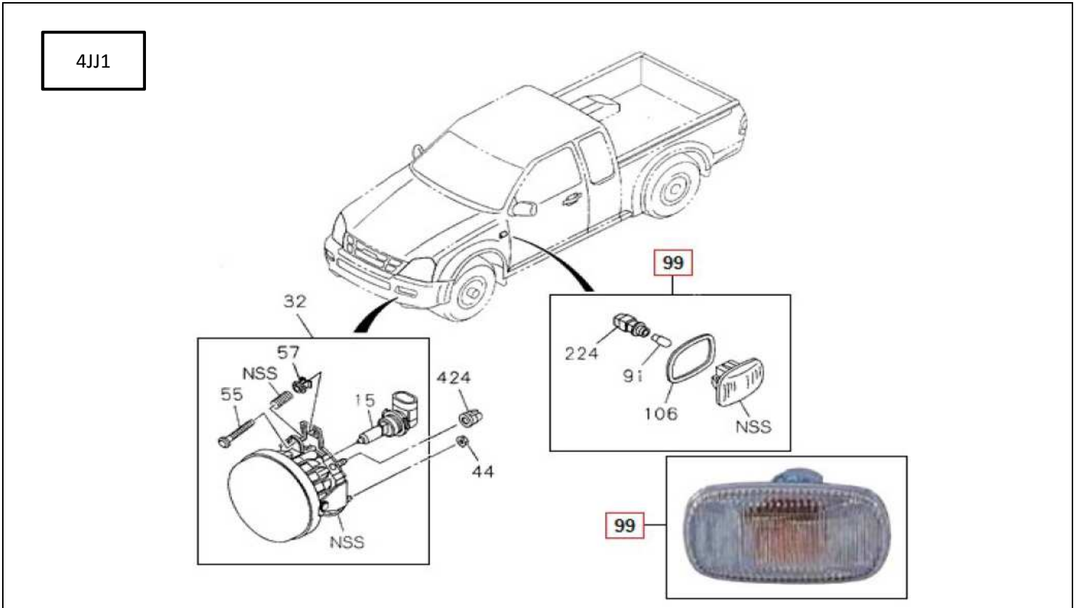
FIG.NO : 8-01 LAMP; FRONT AND FRONT SIDE
