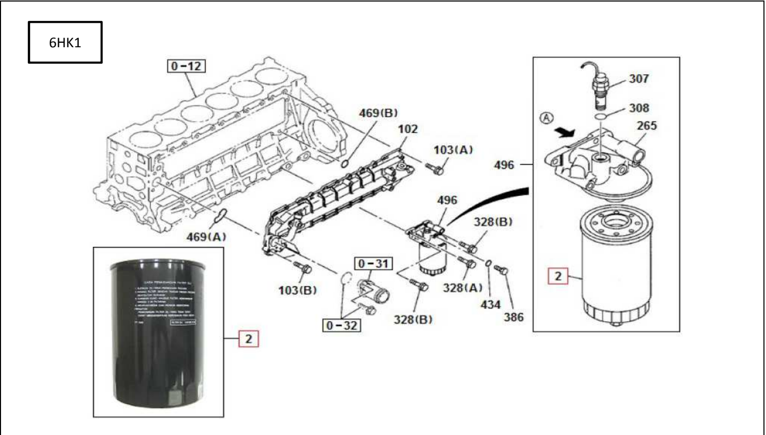
FIG.NO : 0-50 OIL COOLER AND OIL FILTER
