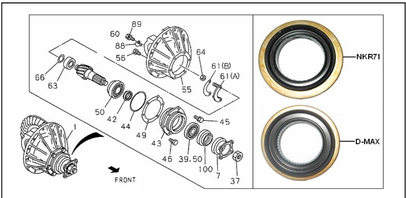
FIG.NO : 4-25 REAR FINAL DRIVE
