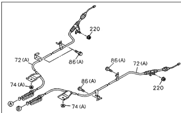
FIG.NO : 3-11 PARKING BRAKE CONTROL
