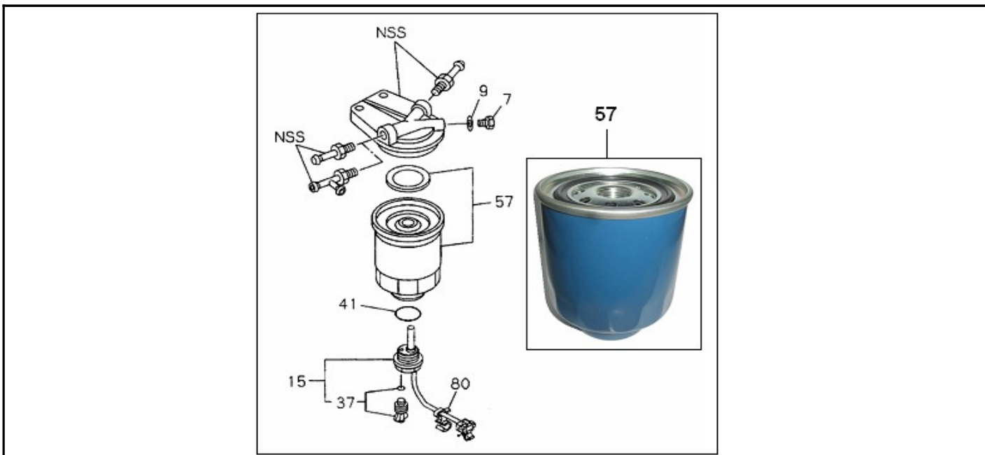
FIG.NO : 1-45 WATER SEDIMENTER FUEL
