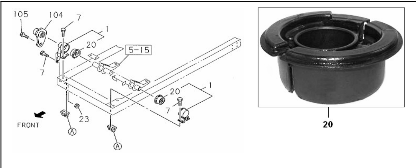
FIG.NO : 5-10 RUBBER MOUNTING CAB BRKT
