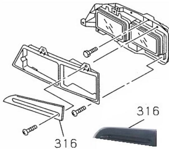
FIG.NO : 8-01 LAMP; FRONT AND FRONT SIDE
